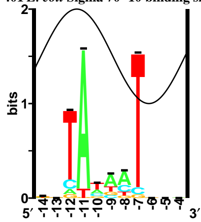
401 E. coli Sigma 70 -10 binding sites
